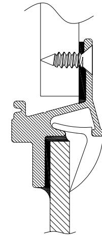
OPTIONAL BOLT-ON INSTALLATION
