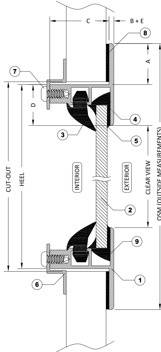
SECTION A-A WITH CLAMP IN INSTALLATION
