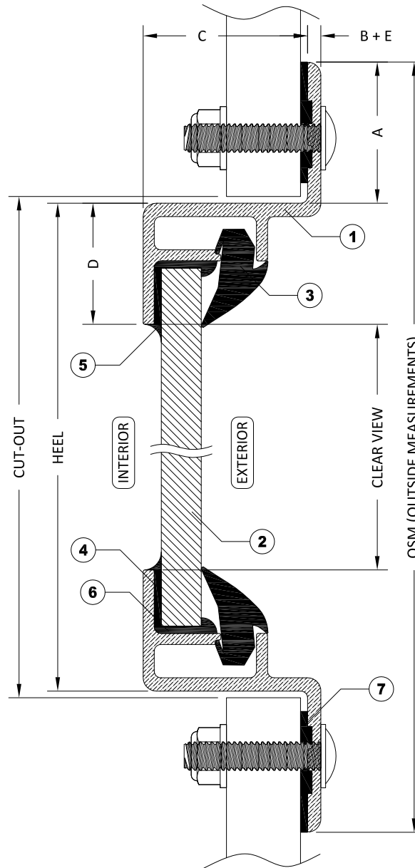
SECTION A-A WITH BOLT-ON INSTALLATION
