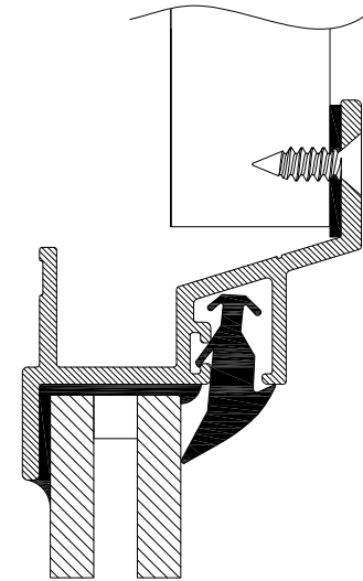
OPTIONAL BOLT-ON INSTALLATION
