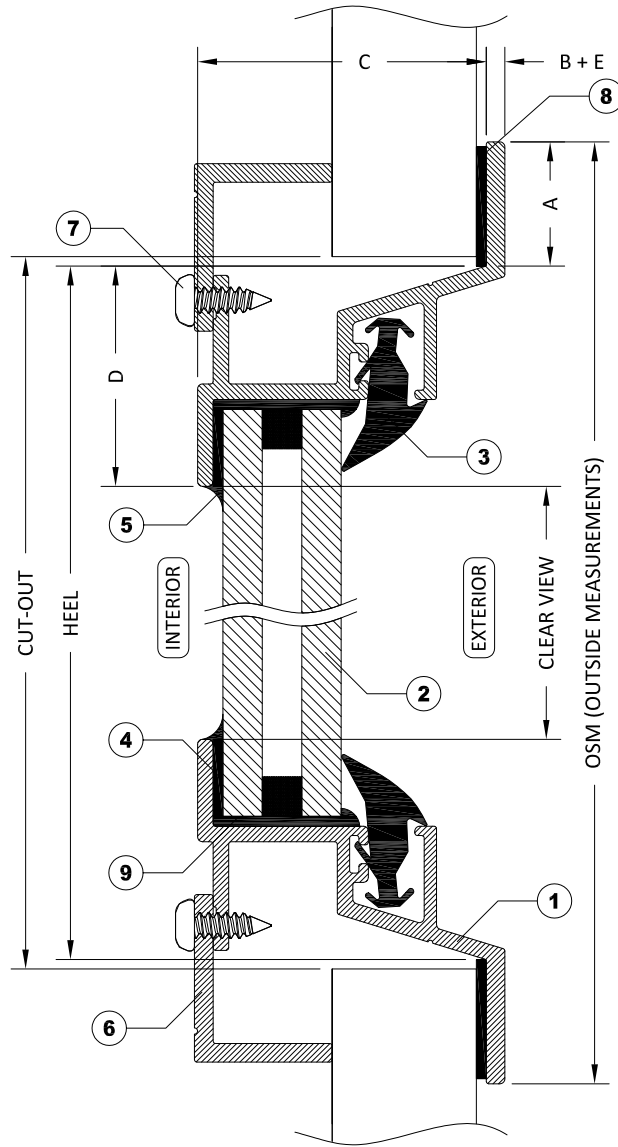
SECTION A-A WITH CLAMP IN INSTALLATION
