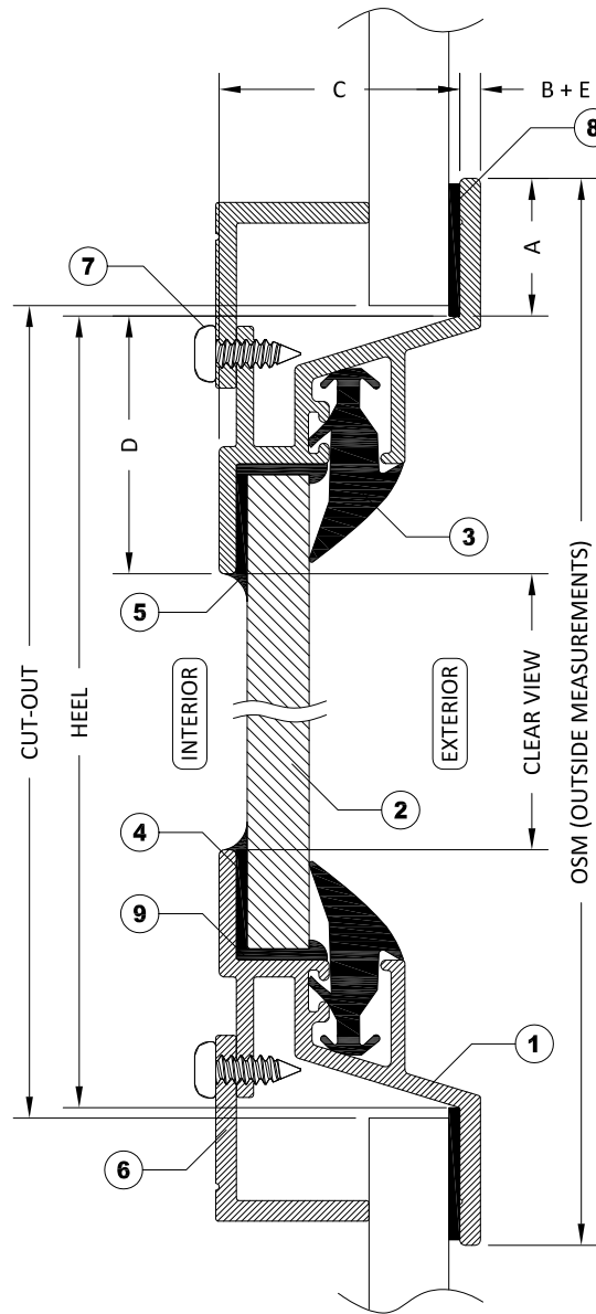
SECTION A-A WITH CLAMP IN INSTALLATION
