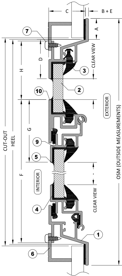
SECTION B-B WITH CLAMP IN INSTALLATION
