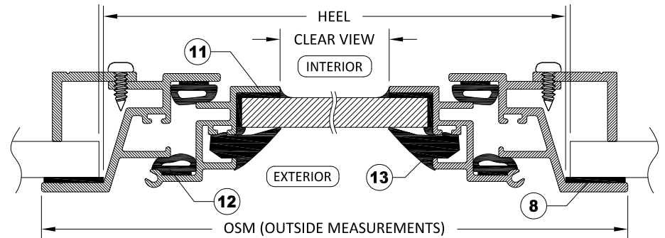
SECTION A-A WITH CLAMP IN INSTALLATION
