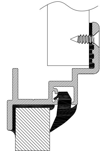
OPTIONAL BOLT-ON INSTALLATION
