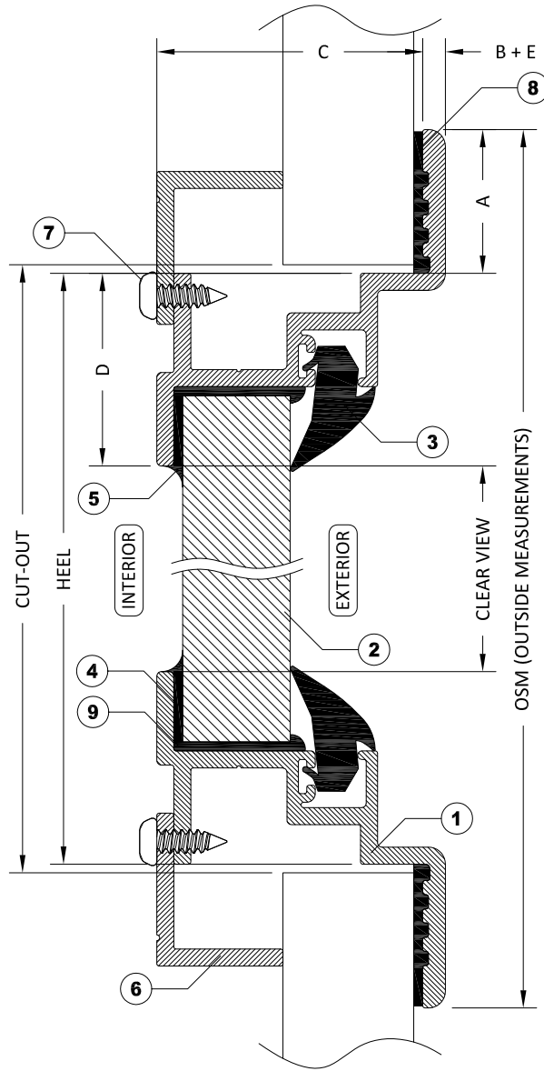
SECTION A-A WITH CLAMP IN INSTALLATION
